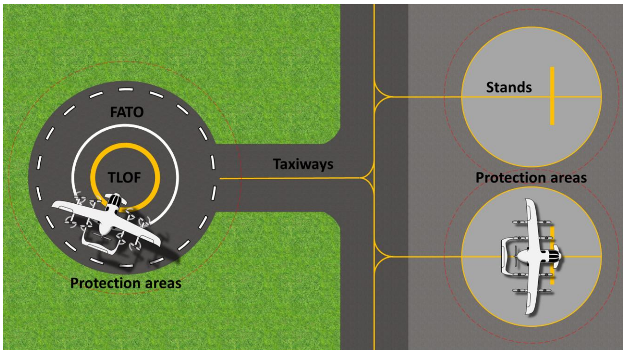
Figure 1 – Vertiport components
