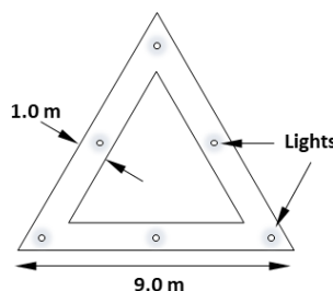
Figure 19 – Arrangement for aiming point lights
