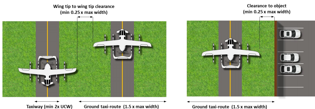
Figure 3 - VCA taxiways and clearance distances
